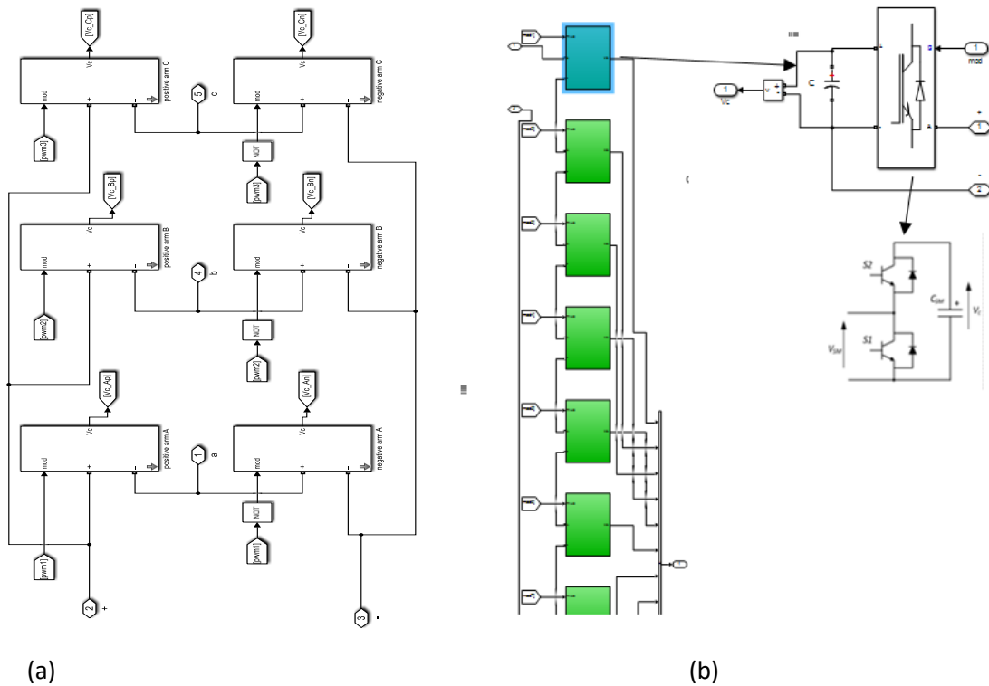
Figure 3. MMC Structure, (a) The MMC Structure, (b) the arm structure (left) 12 cell structure (right) with half-bridge cell structure
